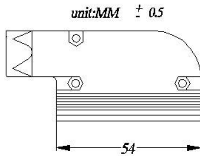
Thumbscrew H07-DAR
